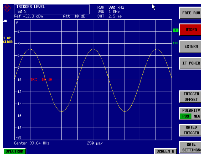
Fig. 2.21 Demodulated FM signal
