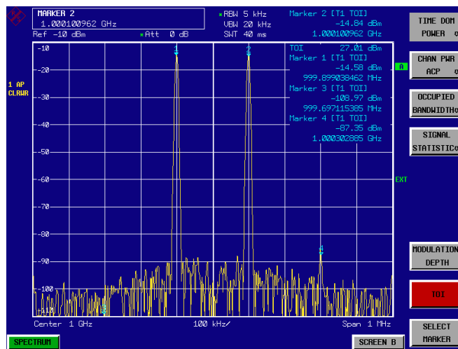
Fig. 2.3 Result of intrinsic intermodulation measurement on the R&S FSU. The 3 rd order intercept (TOI) is displayed at the top right corner of the grid
