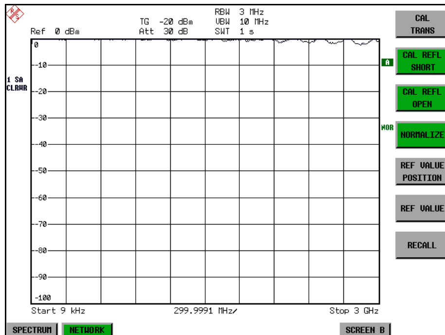
Fig. 4.30 Normalized display
