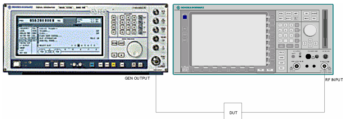
Fig. 4.28 Test setup for transmission measurement
