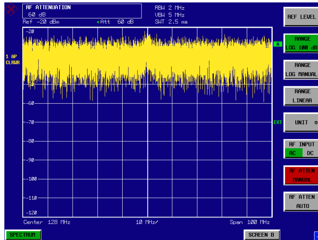
Fig. 2.9 Sinewave signal with low S/N ratio. The signal is measured with the autpeak detector and is completely swamped by the intrinsic noise of the R&S FSU.
