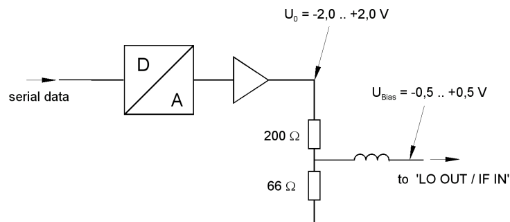
Fig. 4.36 Bias circuit of the R&S FSU
